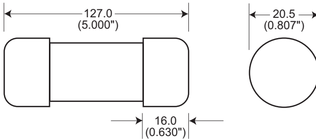
Fig. 1: 2-30 Amp Range
