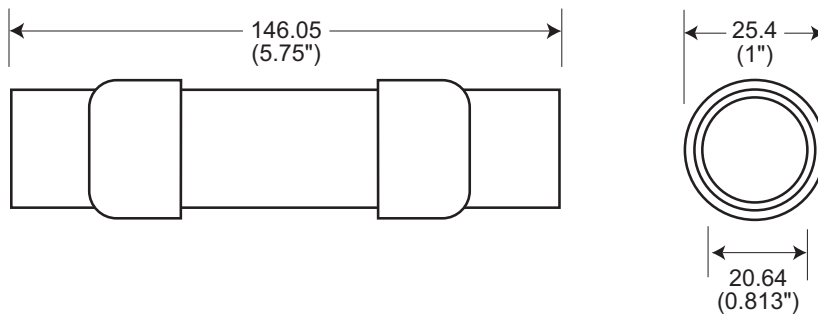
Fig. 2: 35-60 Amp Range
