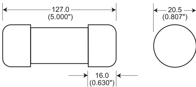
Fig. 2: 35-60 Amp Range
